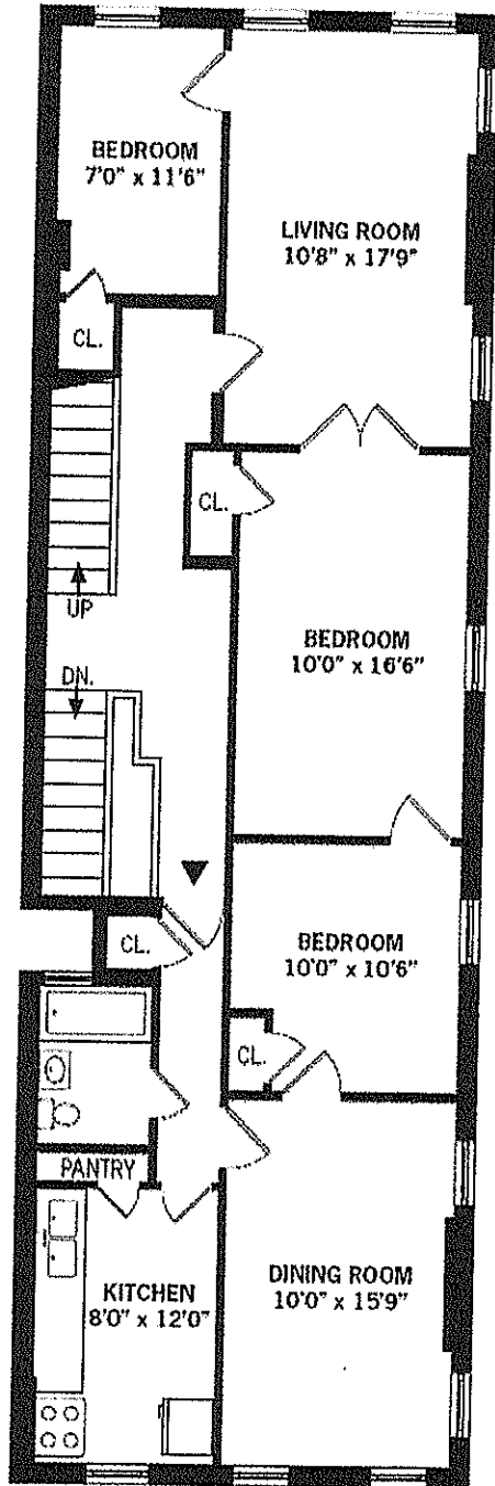
SECOND FLOOR
